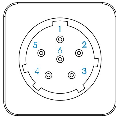
CONN-BA5590 PINOUT (FRONT VIEW)
