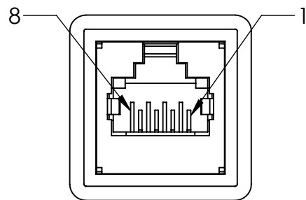
SECTION A-A P1 & P2 PINOUT SCALE 1.5 : 1
