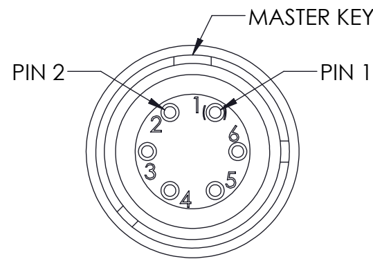
PIN LAYOUT OF P1 AND P2 (FRONT FACE)
